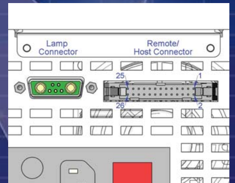
Lamp Unit
