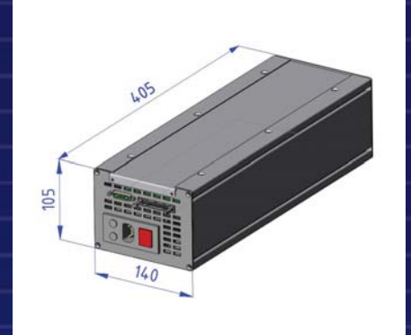
Power Supply
